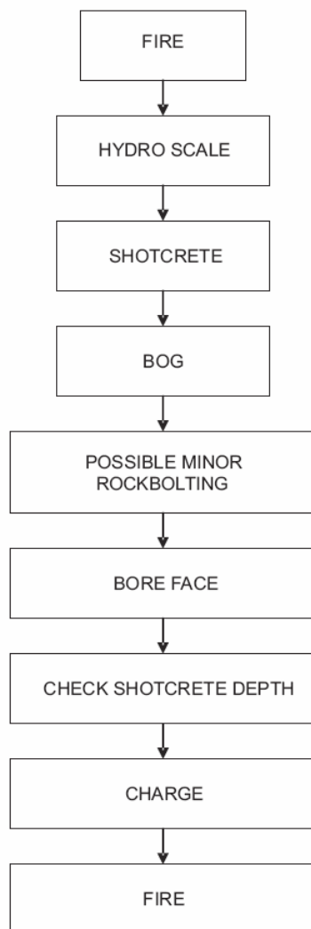
Figure 9 – A proposed fibrecrete cycle
