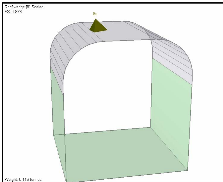
FIG 3 - Fibrecrete with Small Wedge
