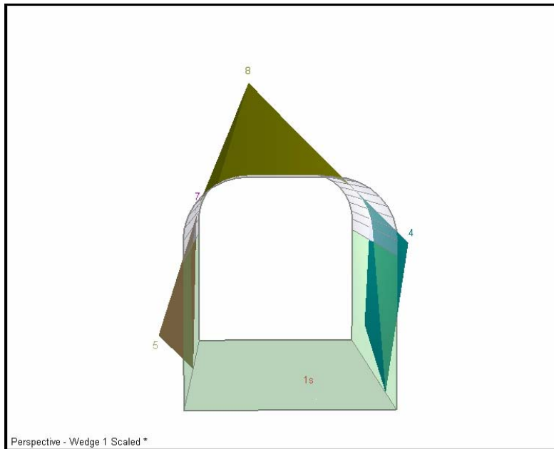
FIG 6 - Back and wall wedges
