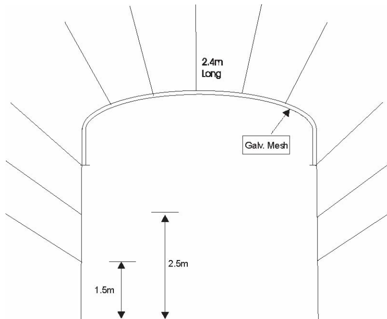
FIG 5– Standard rockbolting and meshing pattern (section view).
