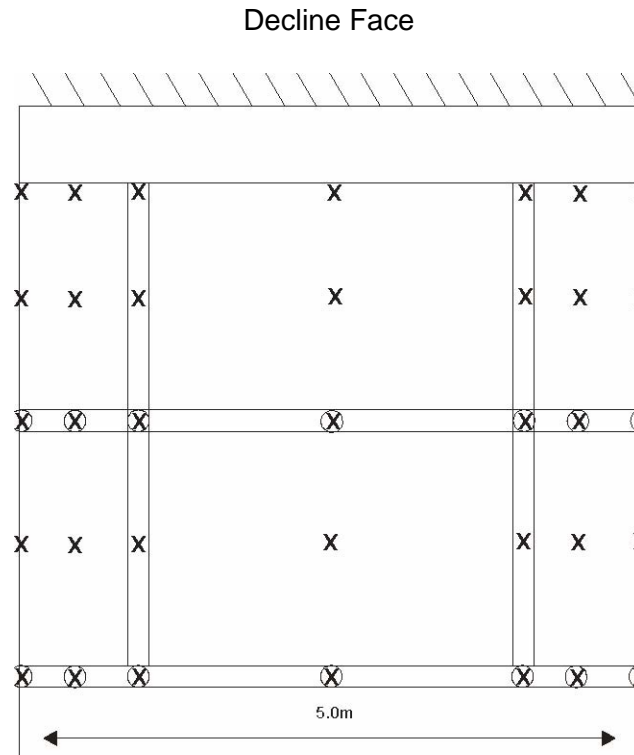
FIG 4 – Standard and rockbolting and meshing pattern (plan view).
