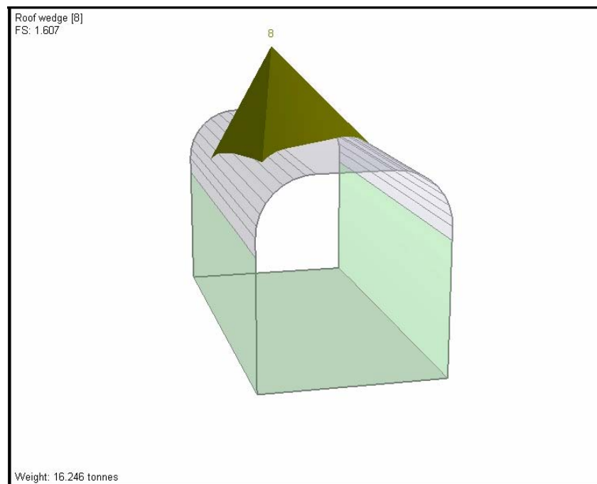
FIG 2 -Standard Fibrecrete Pattern
