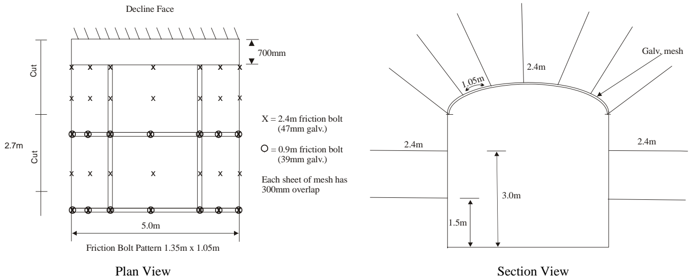
Fig. 1 Typical Bolting Pattern with Mesh
